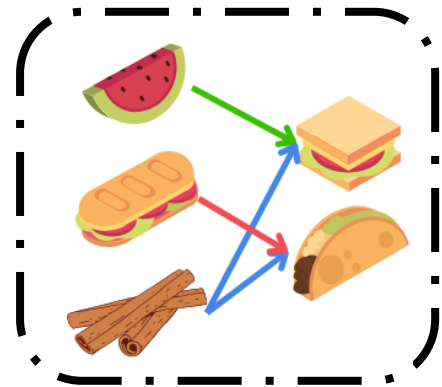
Causal relationships
